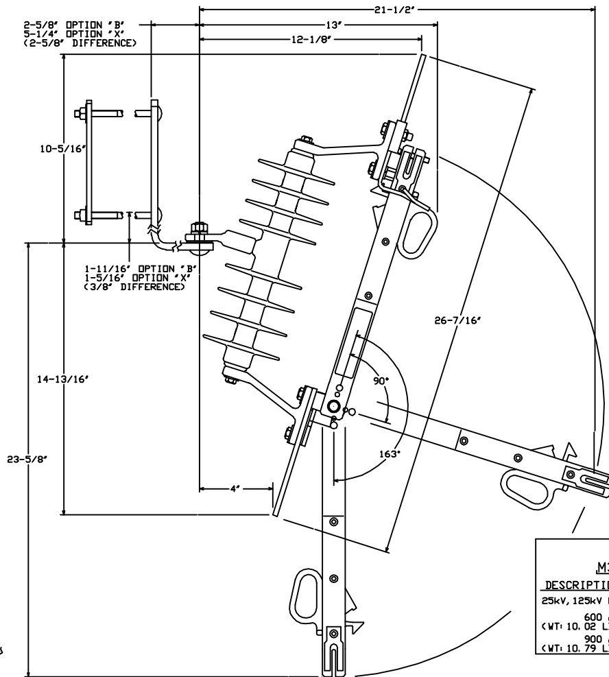
OPTION "P" PARALLEL GROOVE TERMINALS CONSIST OF 2 EACH CONNECTORS & HARDWARE FOR #2-500 KCMIL COPPER OR ALUMINUM CONDUCTOR
